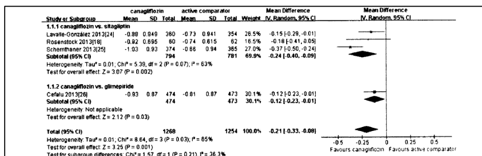
Fig. 3 Meta-analysis for HbA1c change from baseline, canagliflozin versus active comparator
