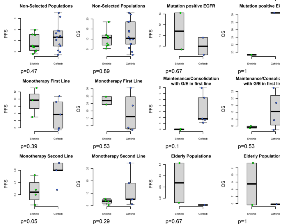
Figure S8: Efficacy analysis in all studies and in various subgroups
